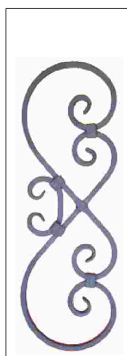
UP080 12mm Square Bar Dim 105 x 900mm
