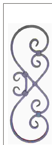
UP081 12mm Square Bar Dim 105 x 900mm
