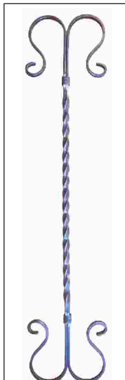
UP087 12 x 6mm Flat Bar Dim 190 x 900mm
