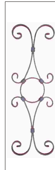
UP098 12 x 6mm Flat Bar Dim 230 x 700mm
