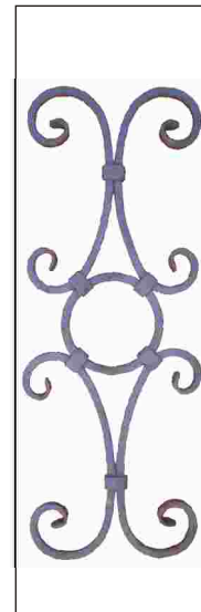
UP029 12mm Square Bar Dim 230 x 700mm
