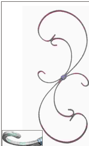
UP024B ~ 12 x 6mm Flat Bar UP024C ~ 16 x 6mm Flat Bar UP024D ~ 20 x 6mm Flat Bar UP024E ~ 25 x 6mm Flat Bar Dim 300 x 750mm
